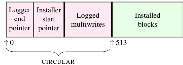
Figure 8: The physical write-ahead log.
